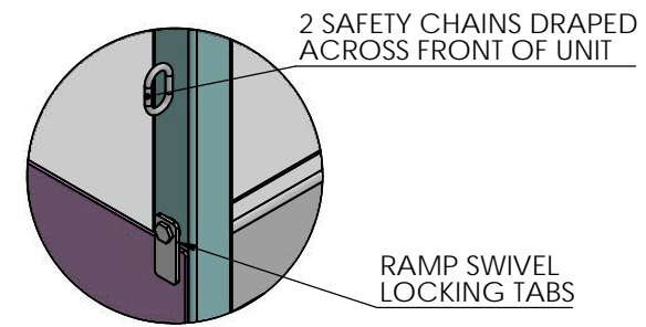
DETAIL C SCALE 1 : 4
